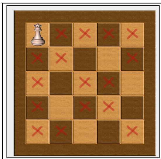
Figure 2 - Inserting the first queen
