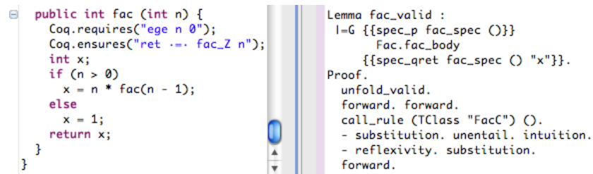
Fig. 1. Java and Coq editor side-by-side; closeup of Coq editor in Fig 2
