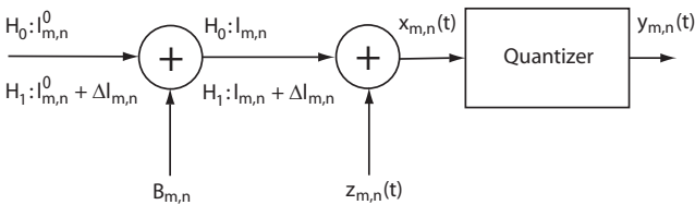
Figure 3: The received signal model
