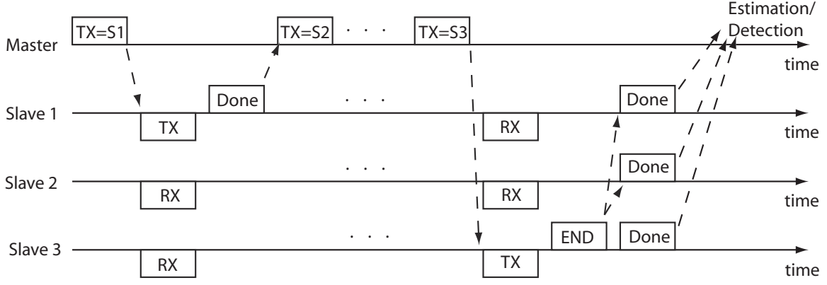
Figure 2: The timing diagram of one scanning cycle
