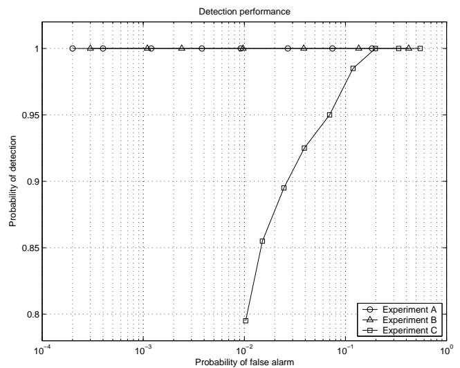
Figure 5: The detector performance
