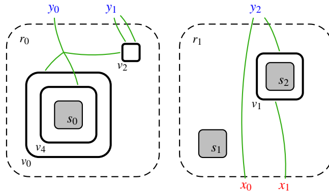
Figure 1: A pure bigraph
