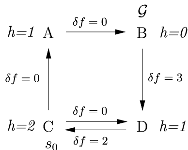
Fig. 4. The example search problem with \delta f costs.
