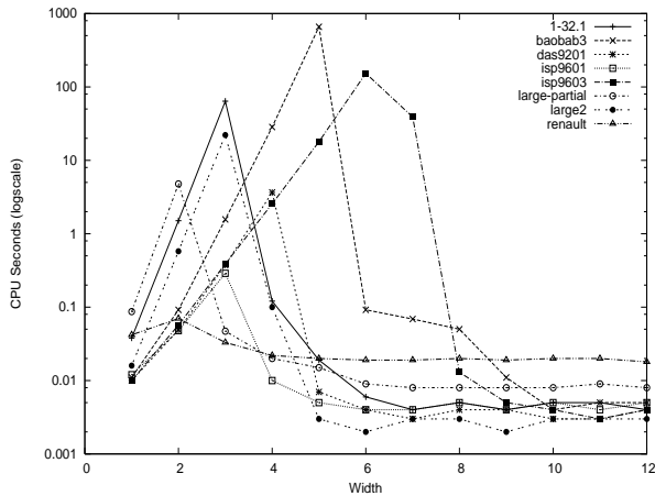
Figure 3: Width vs. CPU-time (y axis in logscale). The empirical complexity peaks at k^* - 1 .
