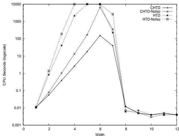
Figure 4: The effect of detecting isomorphism and CHTD vs. HTD in isp9603 instance (time limit 10000 seconds).
