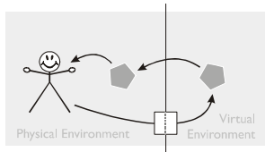
Fig. 4. Virtual→physical action [2]
